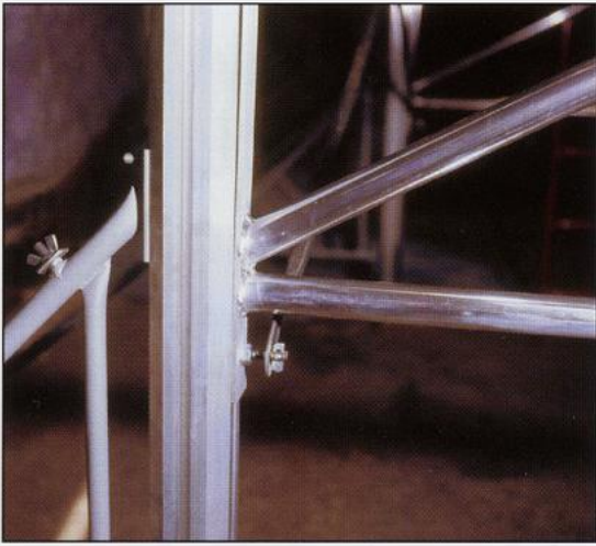
SIMPLE "T-BOLT" CONNECTION (FRAME, LEGS & PANELS ARE PREASSEMBLED)
